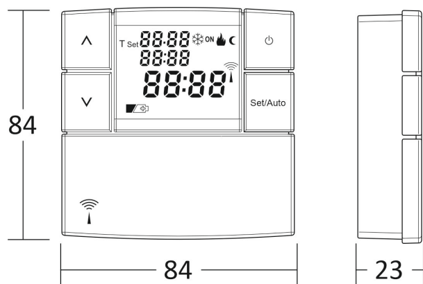
Dimensions (mm)
